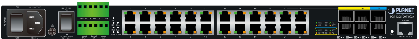
Figure 2-1: IGS-5225-20T4C2X Switch Front Panel
