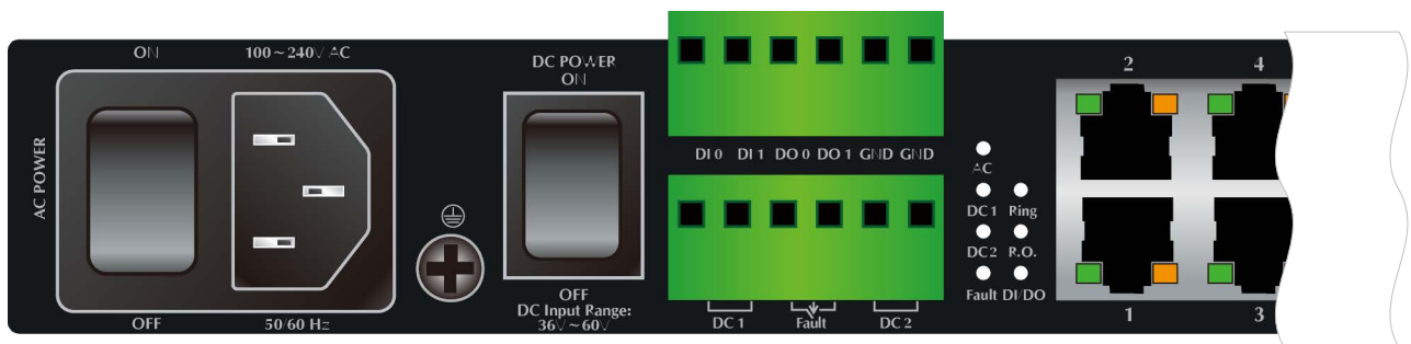
Figure 2-9: IGS-5225-16T4S LED on Front Panel
